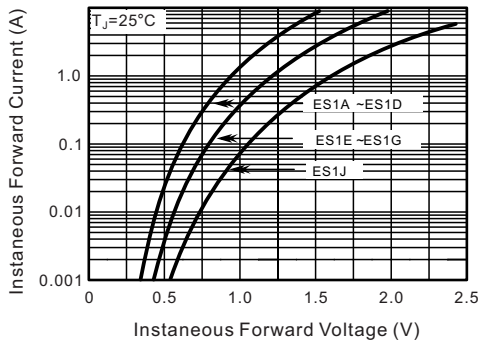
FIG.1-TYPICAL FORWARD CHARACTERISTICS
