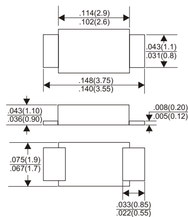
SOD123FL
